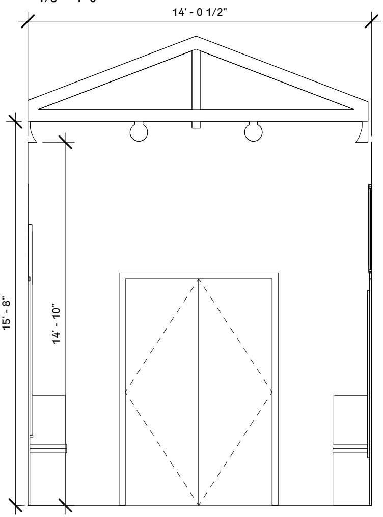
2 HALLWAY - ELEVATION B 1/4" = 1'-0"
