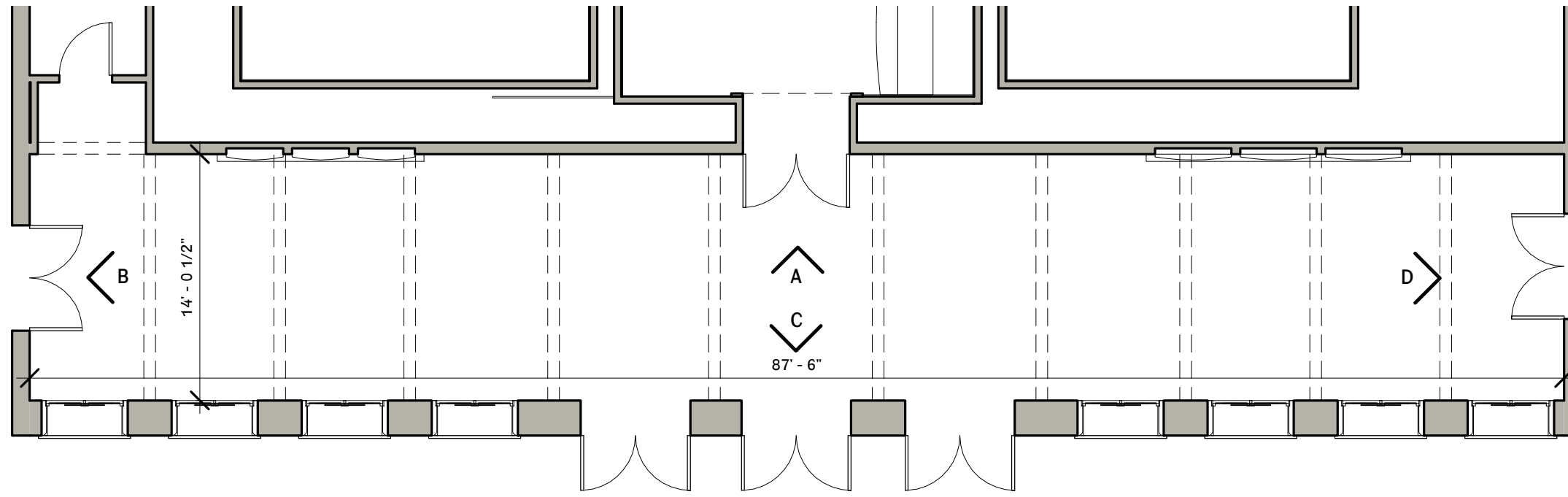
1 ENTRY HALLWAY PLAN 1/8" = 1'-0"
