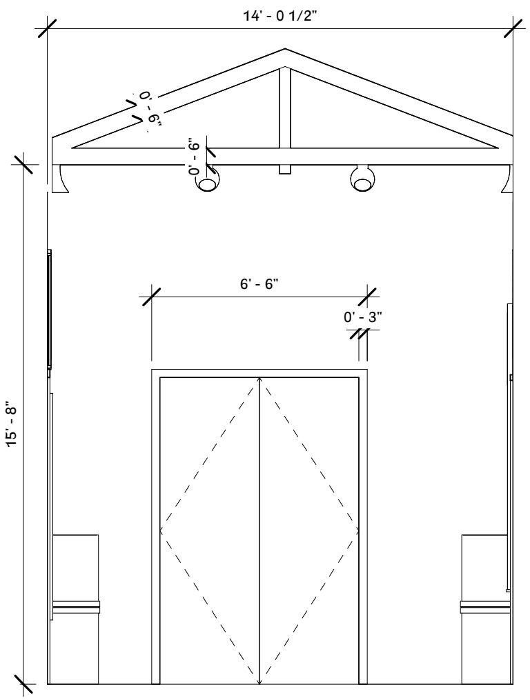
3 HALLWAY - ELEVATION D 1/4" = 1'-0"
